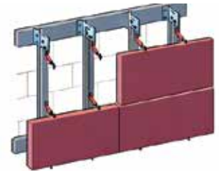
Profile Horizontal Connection
