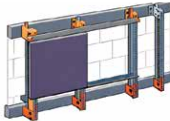
Profile Connections for Thin Stones
